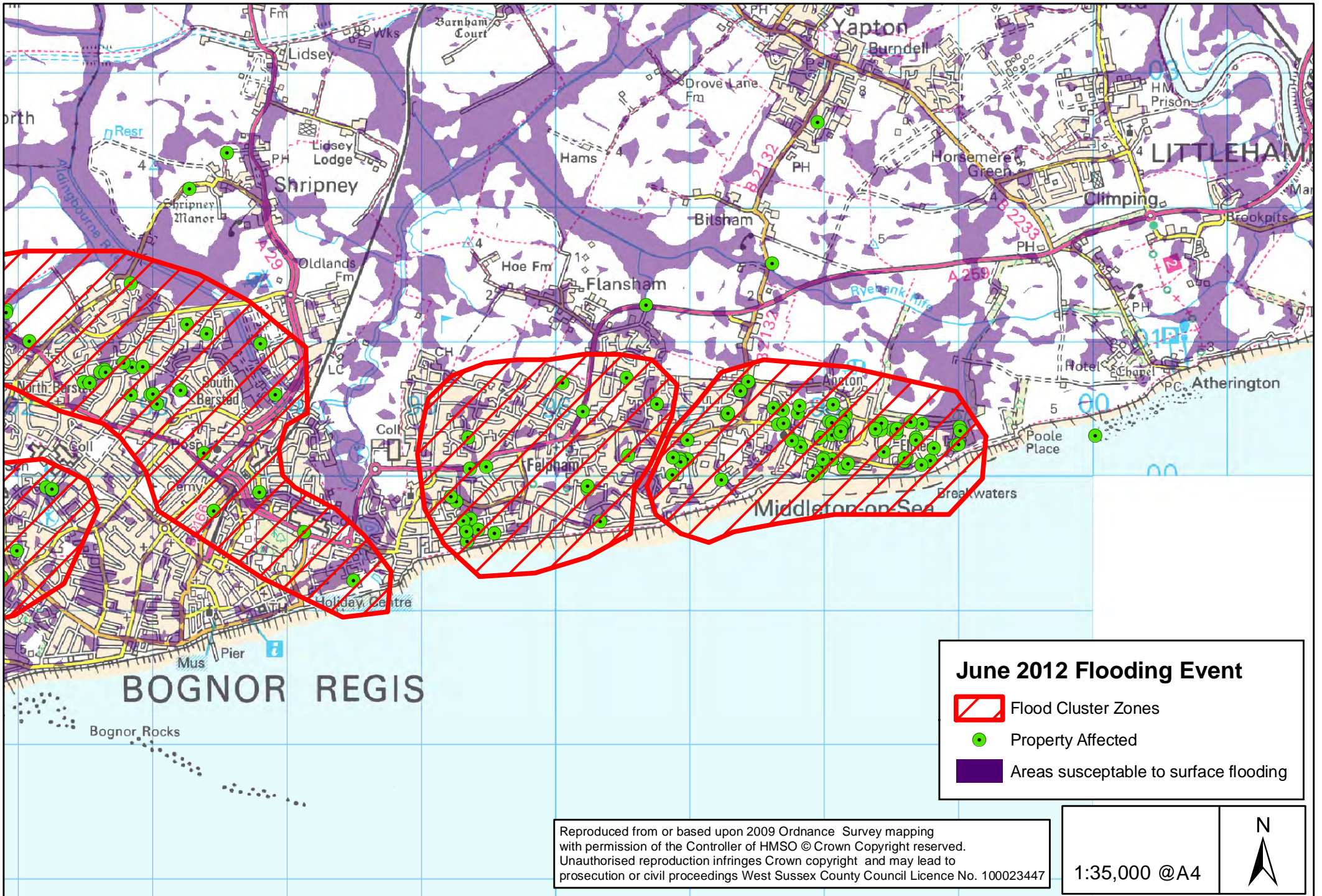
Figure 7. 'Clusters 1 and 2' - Areas Susceptible to Surface Water Flooding.
