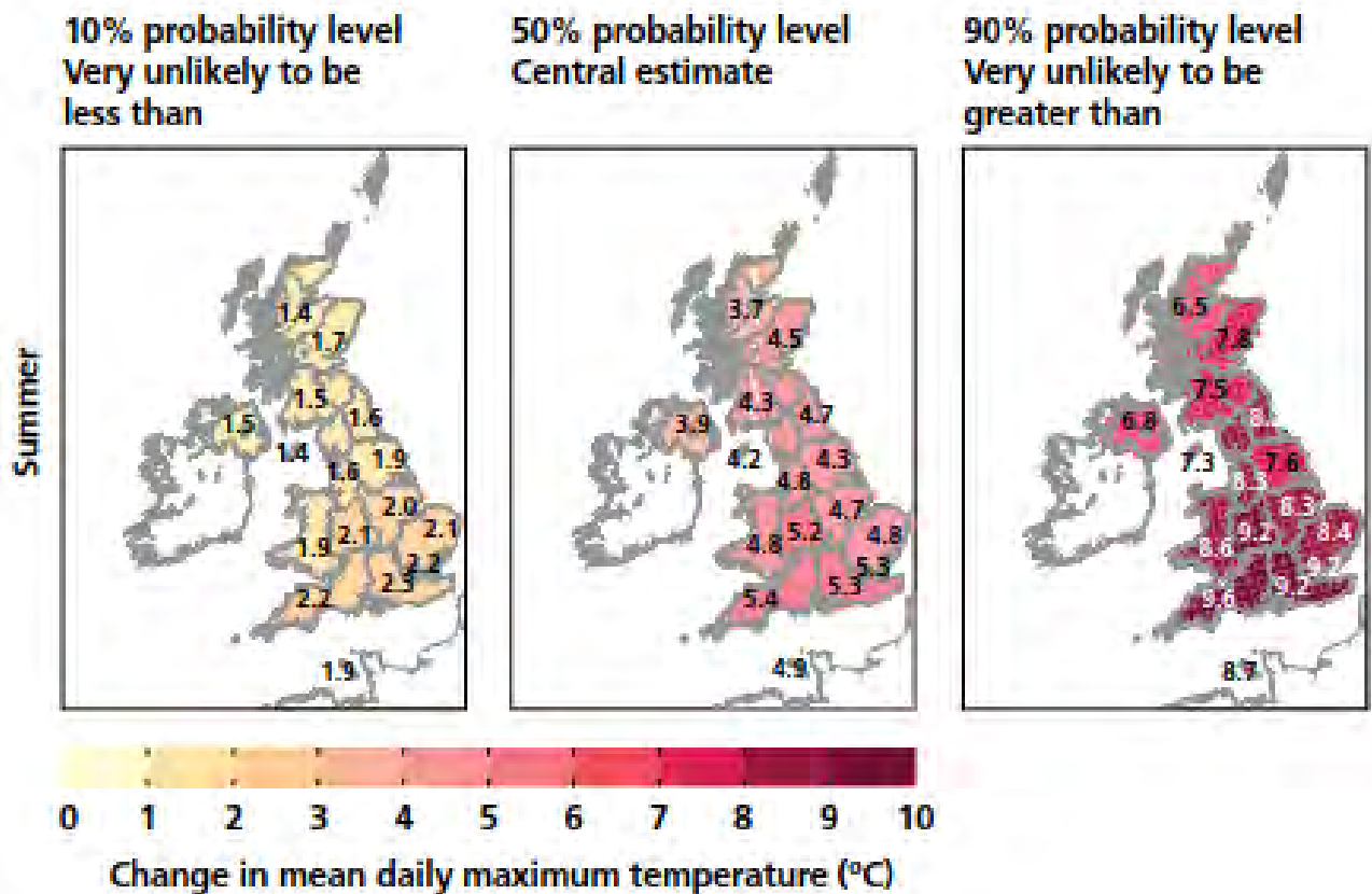
Figure 3-7 - 10, 50 and 90% Probability Levels of Changes to Summer Mean Daily Maximum Temperature Averaged Over Administrative Regions by the 2080s, Under the Medium Emissions Scenario
